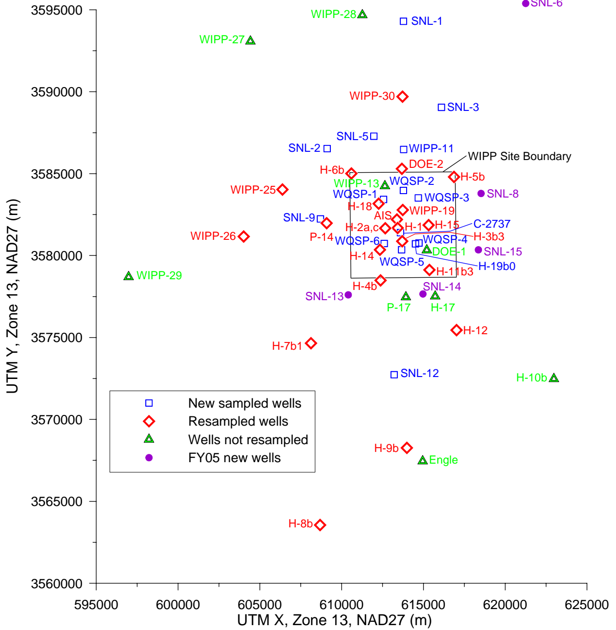
Figure 3. Locations of Culebra wells providing new water-quality information since Siegel et al. (1991a).
